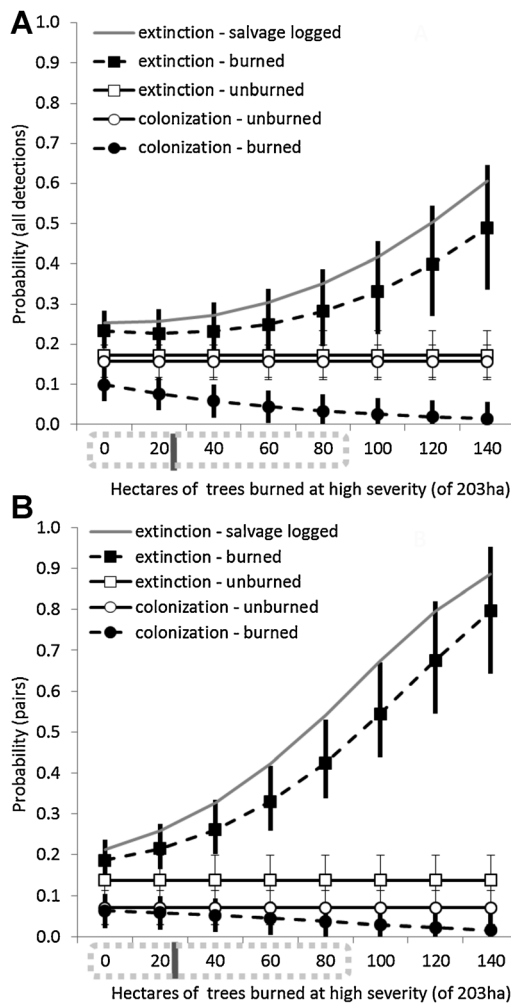
Figure 2. Model-averaged relationship between site colonization and extinction probability and the hectares of owl habitat that burned at high severity within a 203-ha circle around the nest or roost centroid of 71 California spotted owl sites in the San Bernardino and San Jacinto mountains from 2003 to 2011 from all-detection (A) and pairs-only (B) data as calculated from model-averaged beta parameters. Filled symbols and dashed lines are burned owl sites ( \pm SE), open symbols and solid lines are unburned sites ( \pm SE), and solid gray lines represent burned and salvage-logged site extinction probabilities. Vertical gray line in x -axis indicates the mean amount of owl habitat that burned at high severity in all burned sites. Dotted gray rectangle in x -axis indicates 95% confidence interval of amount of owl habitat that burned at high severity in all burned sites. We set individual (site-specific) covariate values to the mean for each covariate.
