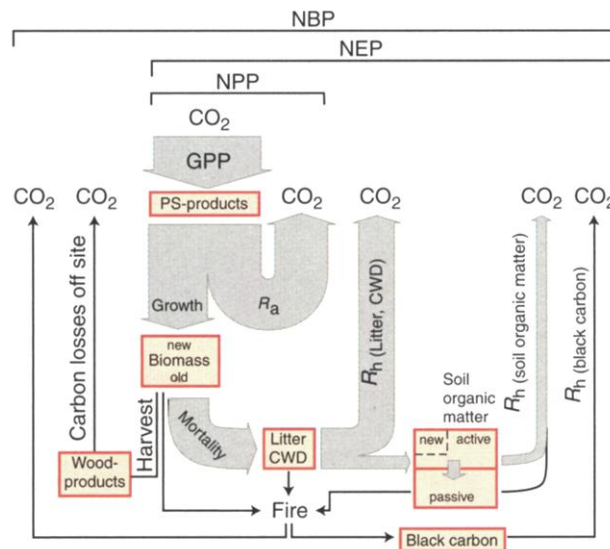
Schematic representation of the terrestrial carbon cycle. Arrows indicate fluxes; boxes indicate pools. The size of the boxes represents differences in carbon distribution in terrestrial ecosystems. CWD, coarse woody debris; R_h , heterotrophic respiration by soil organisms; PS, photosynthesis.
