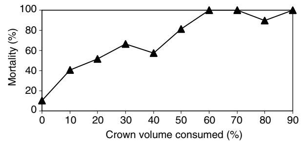
Fig. 4. Observed percent mortality of ponderosa pine 3 years after fire by crown volume consumed for the Side and Bridger-Knoll wildfires in northern Arizona.
