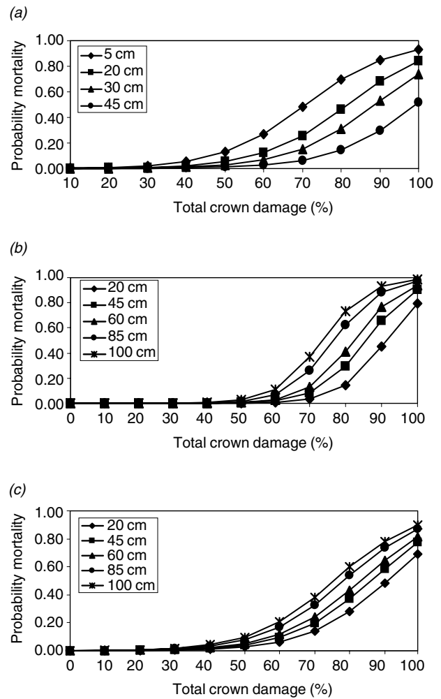
Fig. 8. Distribution of predicted probability of ponderosa pine mortality for logistic regression models using total crown damage and diameter at breast height (dbh) for three fires in northern Arizona. Dauber prescribed fire (a), Side wildfire (b), and Bridger-Knoll wildfire (c). See Table 4 for model form.
