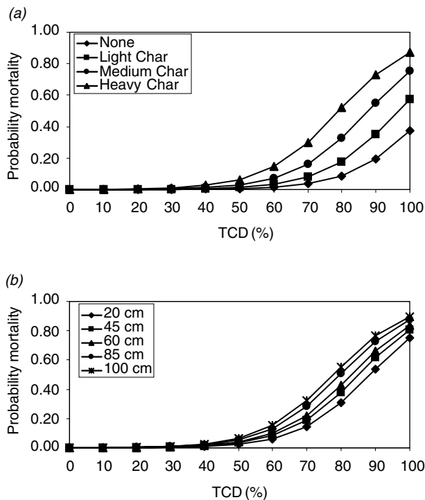
Fig. 9. Distribution of predicted probability of ponderosa pine mortality for logistic regression models using total crown damage (TCD) and bole char severity rating leeward side (CHUPS) (none, light char, medium char, heavy char) (a), and total crown damage (TCD) and diameter at breast height (DBH) (b) for data combined over three fires in northern Arizona. See Table 4 for model form.
