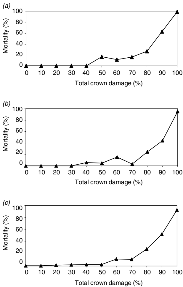
Fig. 5. Observed percent mortality of ponderosa pine 3 years after fire by total crown damage (scorch + consumption) for three fires in northern Arizona. Dauber prescribed fire (a), Side wildfire (b), and Bridger-Knoll wildfire (c).
