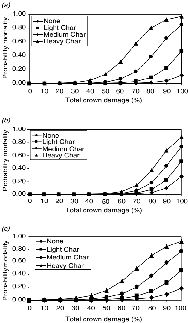
Fig. 7. Distribution of predicted probability of ponderosa pine mortality for logistic regression models using total crown damage and bole char severity rating leeward side (CHUPS) (none, light char, medium char, heavy char) for three fires in northern Arizona. Dauber prescribed fire (a), Side wildfire (b), and Bridger-Knoll wildfire (c). See Table 4 for model form.
