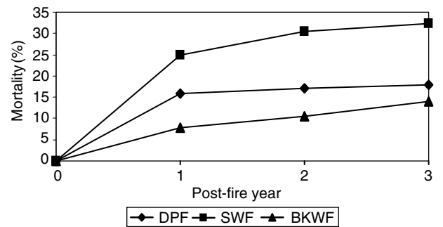
Fig. 6. Observed 3-year post-fire cumulative mortality (%) of ponderosa pine for three fires in northern Arizona. DPF, Dauber prescribed fire; SWF, Side wildfire; BKWF, Bridger-Knoll wildfire.
