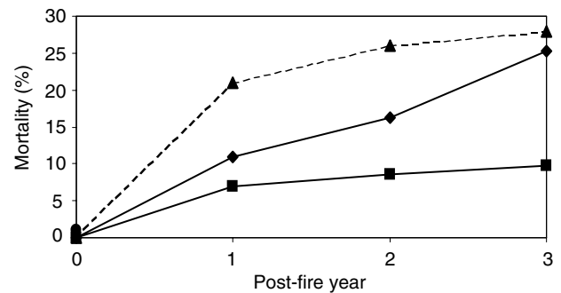
Fig. 10. Percent cumulative ponderosa pine mortality for three post-fire years for the Bridger-Knoll wildfire (solid lines). Data for a summer prescribed fire from Harrington (1993) are represented by dashed line. For the Bridger-Knoll wildfire, squares represent lightly burned areas; diamonds represent severely burned areas.
