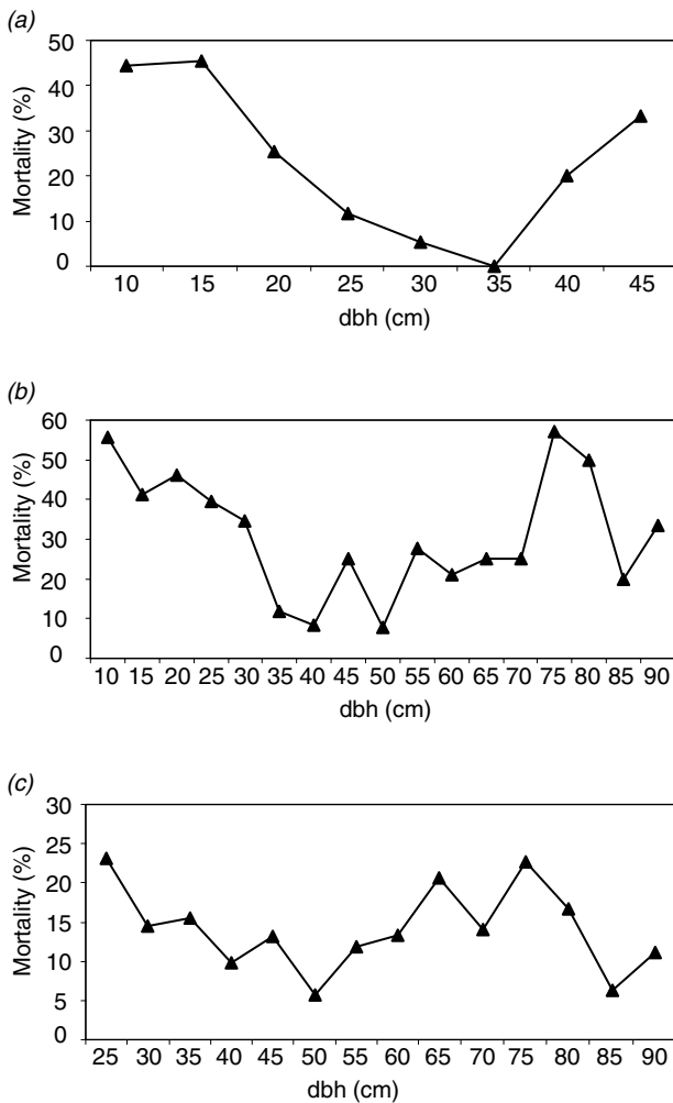
Fig. 2. Observed percent mortality of ponderosa pine 3 years after fire by 5 cm dbh class for three fires in northern Arizona. Sample size range for each dbh class was 3–71 for the Dauber prescribed fire (a), 3–48 for the Side wildfire (b), and 9–109 for the Bridger-Knoll wildfire (c). Data are not shown for dbh classes with <3 trees.
